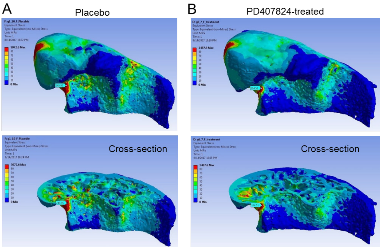
Figure 6 von-Mises stress in response to lateral loading at the condyle edge (BC1). (A) Surface and cross-sectional stresses of the placebo sample. (B) Surface and cross-sectional stresses of PD407824-treated sample.
