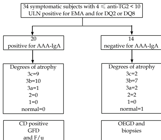
Figure 3 Distribution of AAA-IgA in the 34 subjects of subgroup 3 with anti-TG2 levels comprised between 4 and 10 ULN. CD: coeliac disease; anti-TG2: anti-transglutaminase type 2 antibody; ULN: upper limit of normal; EMA: anti-endomysial antibodies; HLA: human leukocyte antigen; 3a, 3b, 3c, 2, 1 and 0 indicate the grade of intestinal damage according to the Marsh-Oberhuber classification [14,15] ; GFD: gluten free diet; OEGD: oesophagogastroduodenoscopy; F/u: follow-up; AAA-IgA: anti-actin IgA antibody.
